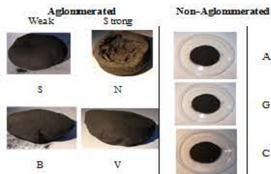
Figure 1. Morphologies of agglomerated and non-agglomerated activated carbons.
