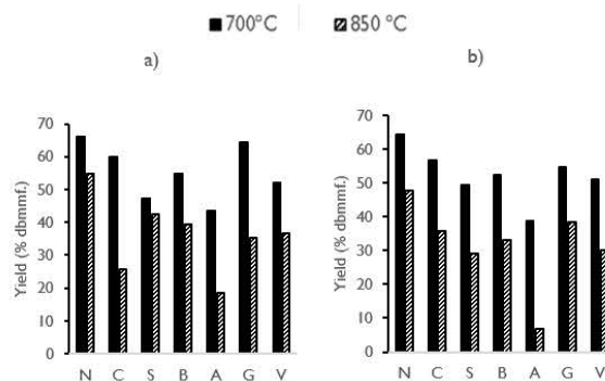
Figure 3. Mass yield of activated carbons from coals : a) 1.5 h; b) 2.5 h.
