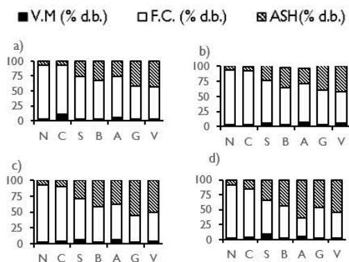
Figure 2. Proximate analysis of activated carbons from coals: a) 700 °C, 1.5 h; b) 700 °C, 2.5 h; c) 850 °C, 1.5 h; d) 850 °C, 2.5 h.
